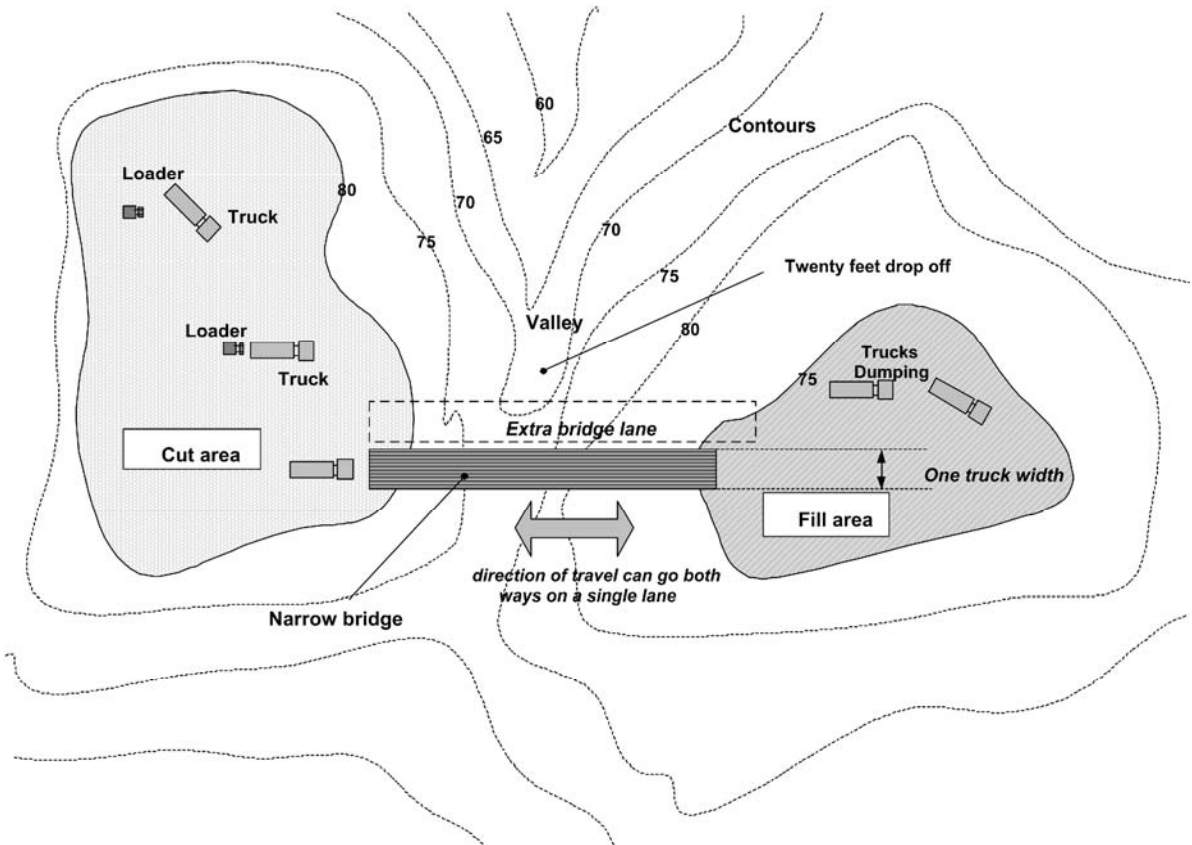
Fig. 6. The developed earth-moving problem schematic
